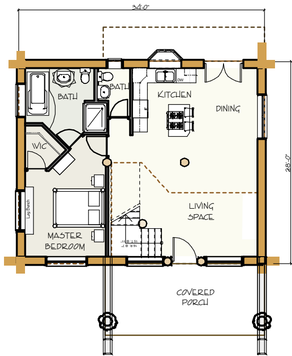
Main Floor
